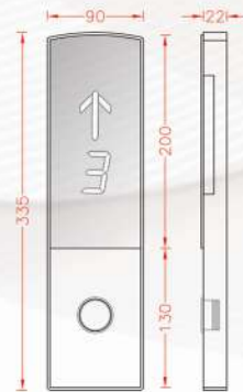
Technical Drawing
