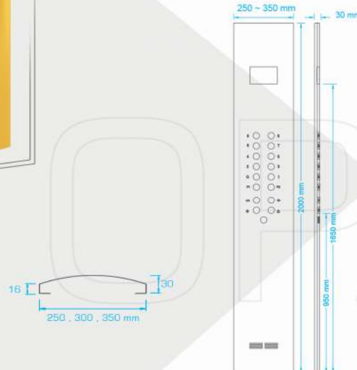
Panel Technical Drawing
